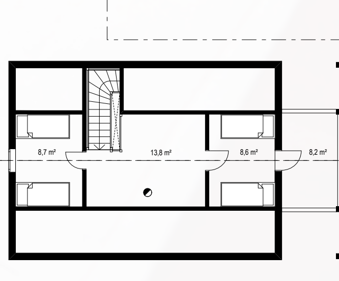
2. Floor 31,1 m 2
