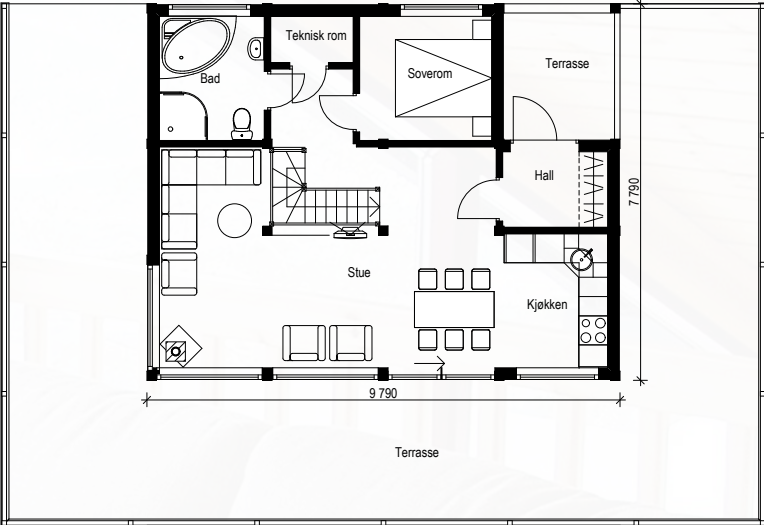
1. Floor 61 m 2
