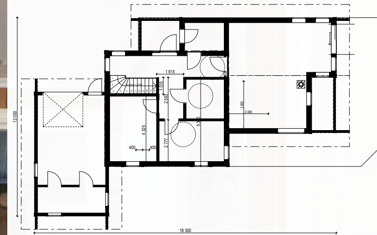
1. Floor 109 m 2
