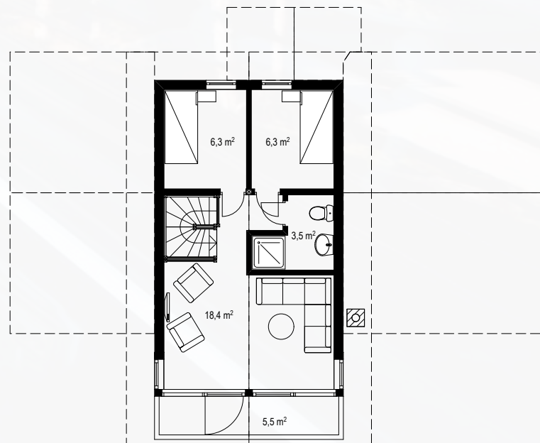
2. Floor 30 m 2
